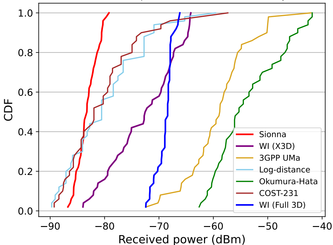
CDF of received power across all EDs (St. Canyon)
