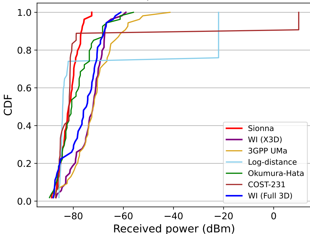
CDF of received power across all EDs (Etoile)
