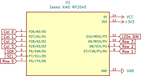
Seeed XIAO RP2040
