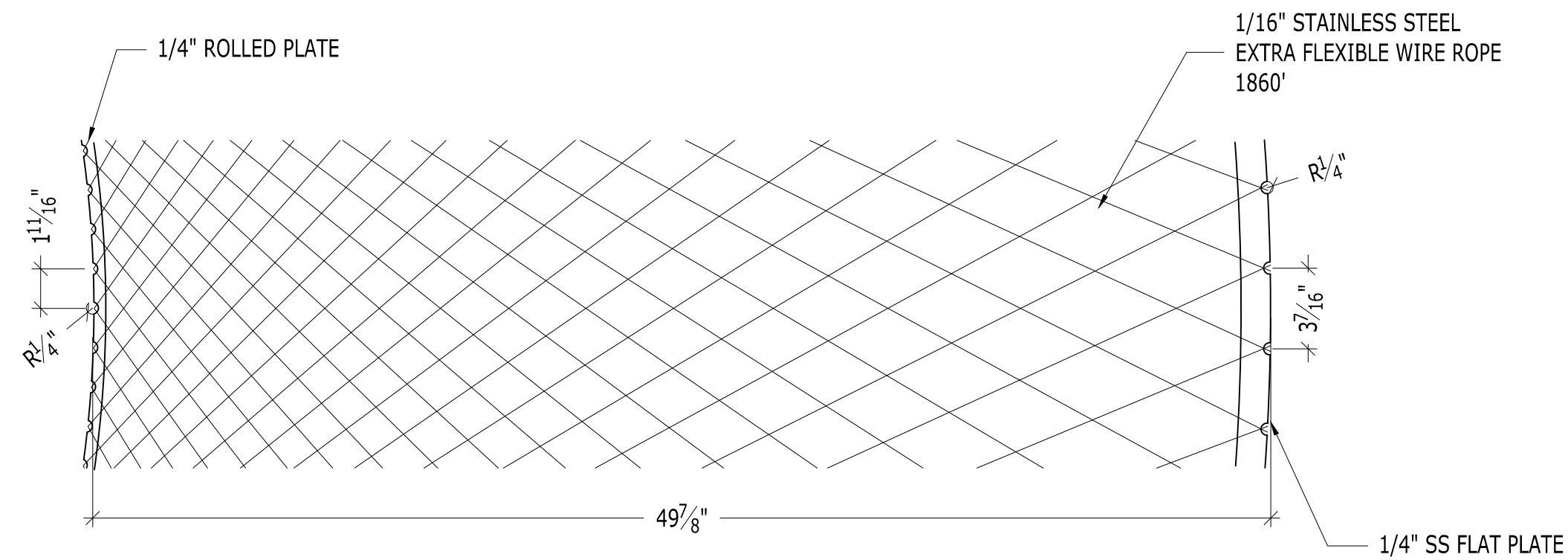
2 DETAIL - WIRE LACE SCALE: 2" = 1'-0"
