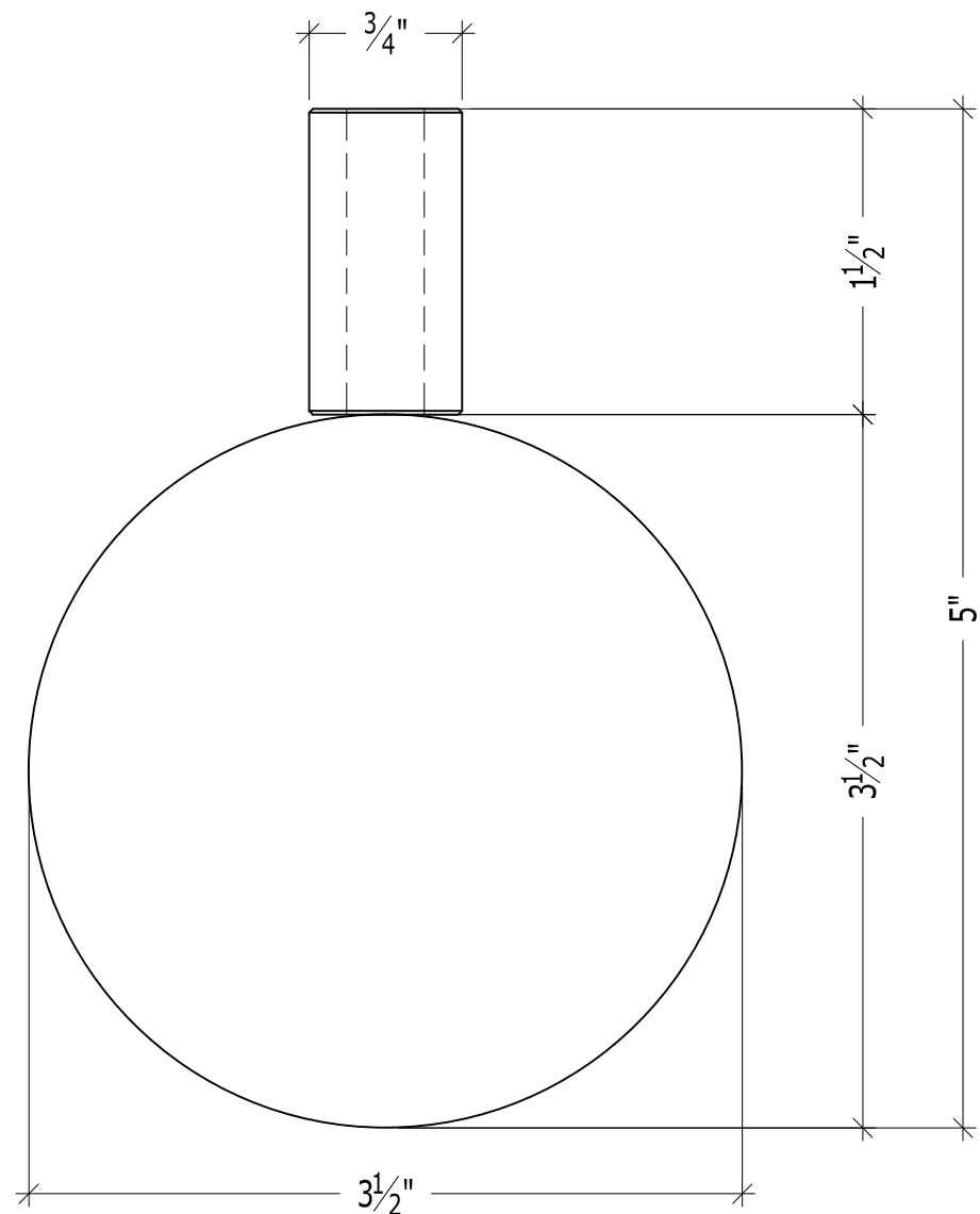
PLAN - SCALE: FULL SCALE
