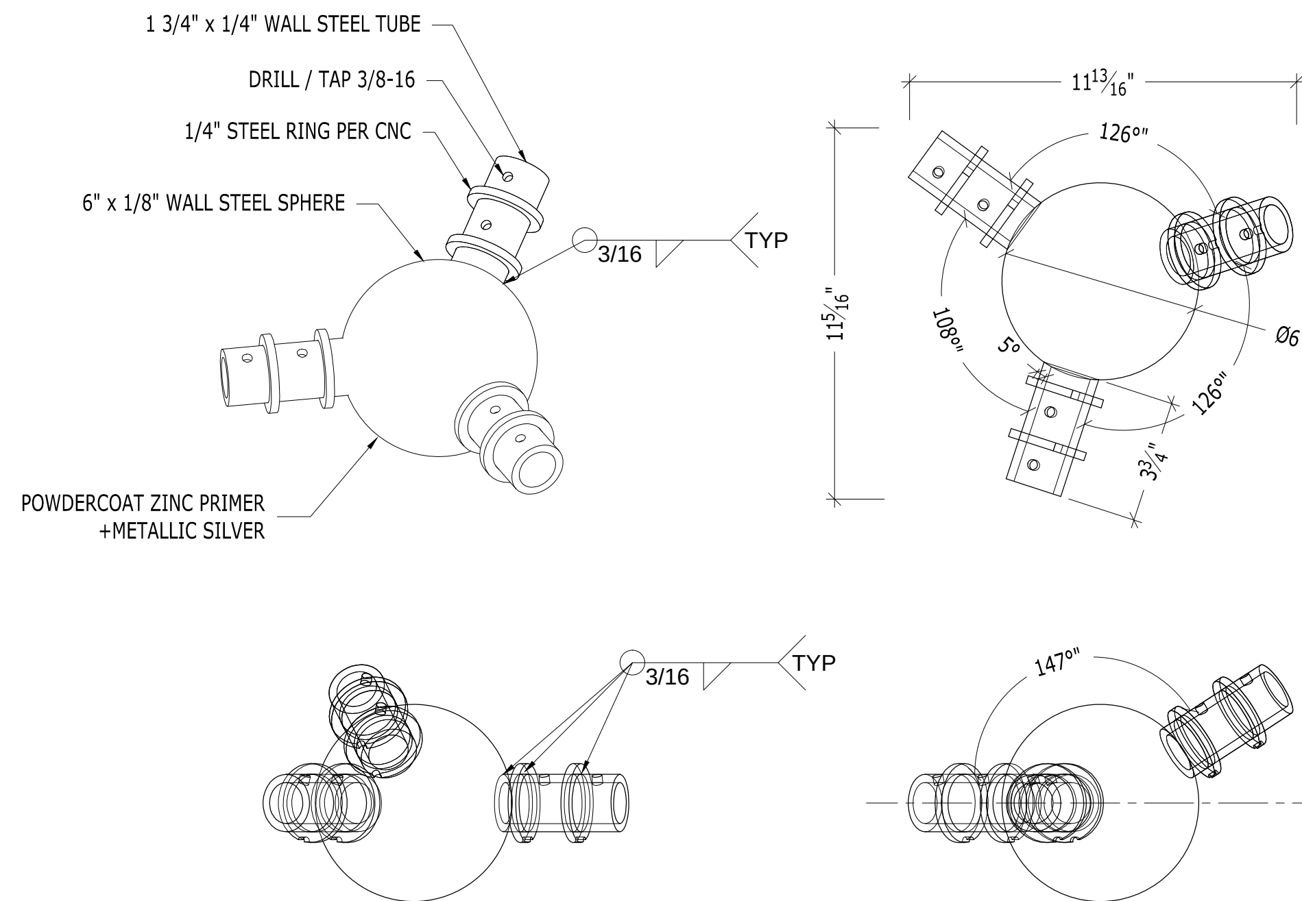
2 DETAIL -VERTEX (55) 7.6 LBS EACH SCALE: 3" = 1'-0"
