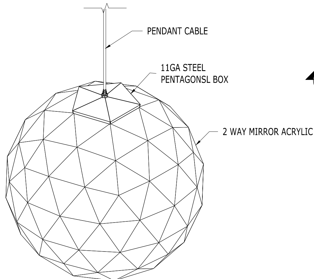
ISO VIEW NTS
