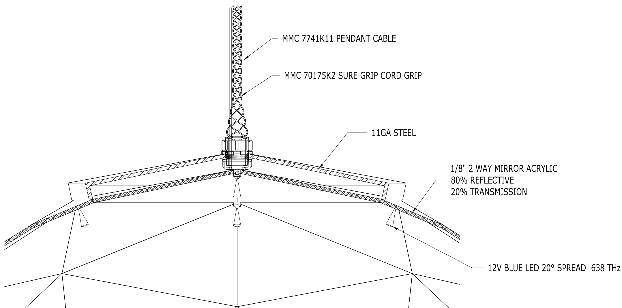
1 SECTION - DETAIL SCALE: HALF SCALE
