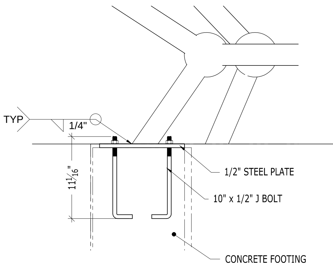
1 DETAIL - FOOTING SCALE: 1-1/2" = 1'-0"
