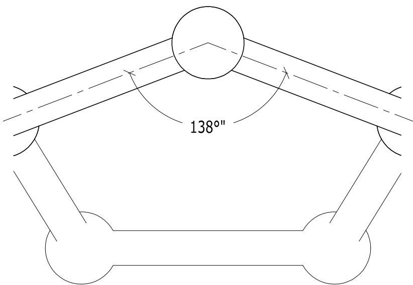
3 DETAIL -HEXAGON TO PENTAGON SCALE: 1-1/2" = 1'-0"
