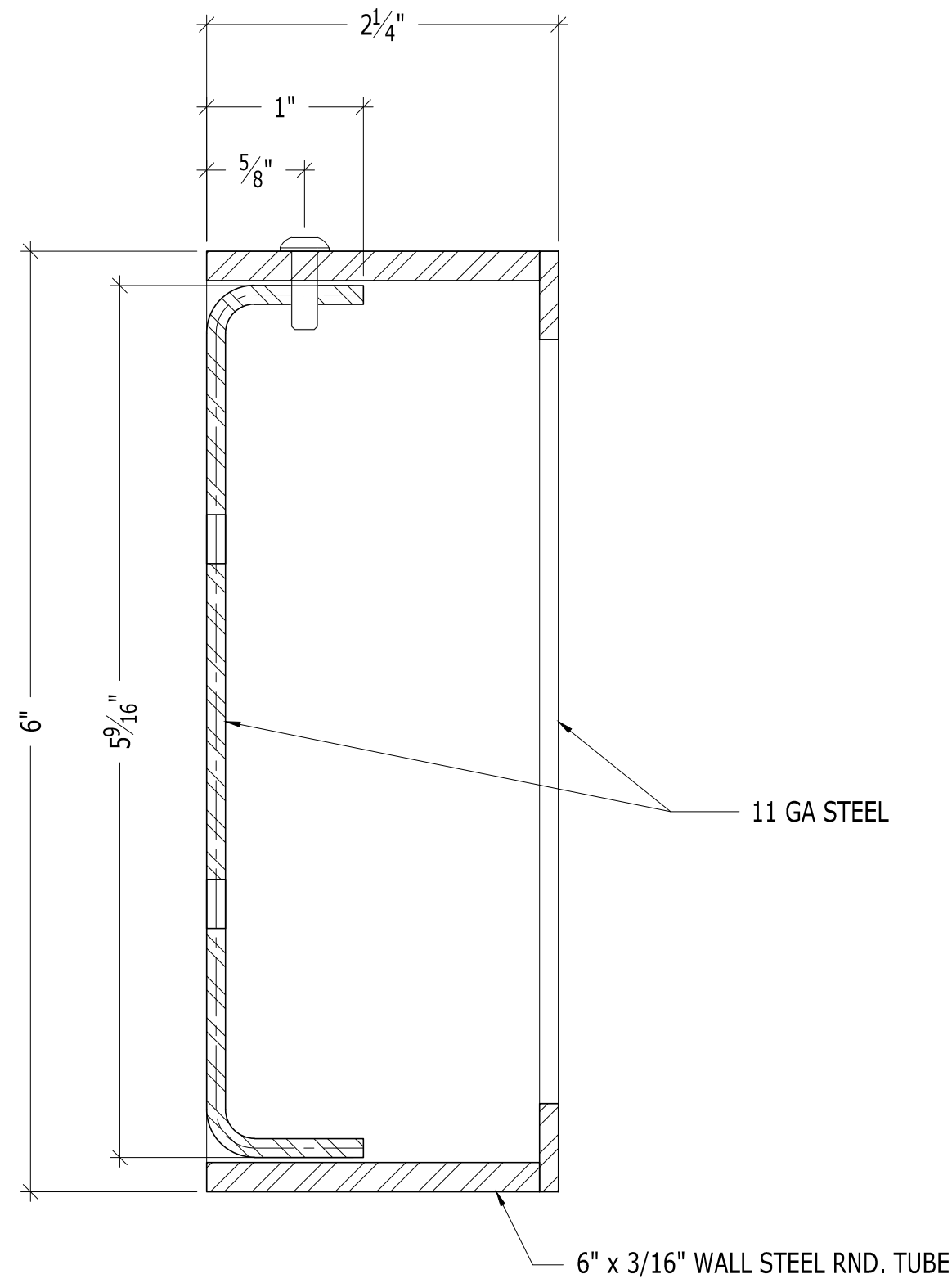
2 SECTION - STEEL SCALE: FULL SCALE
