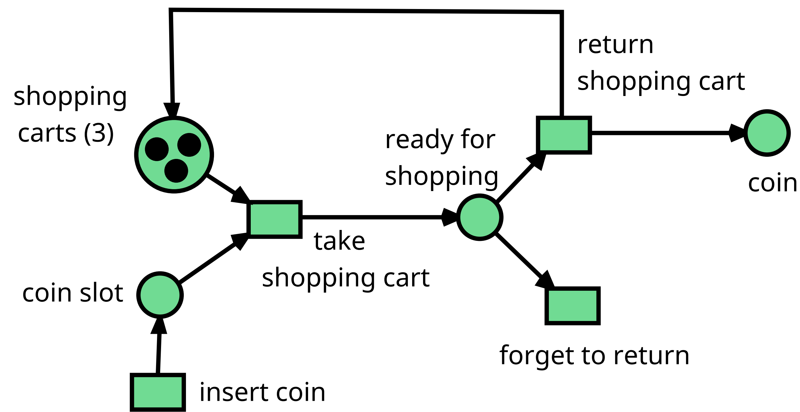
Figure 1: Example of a Petri net consisting of 4 places, 4 transitions, and 3 tokens in one place, modeling a shopping cart rental system
