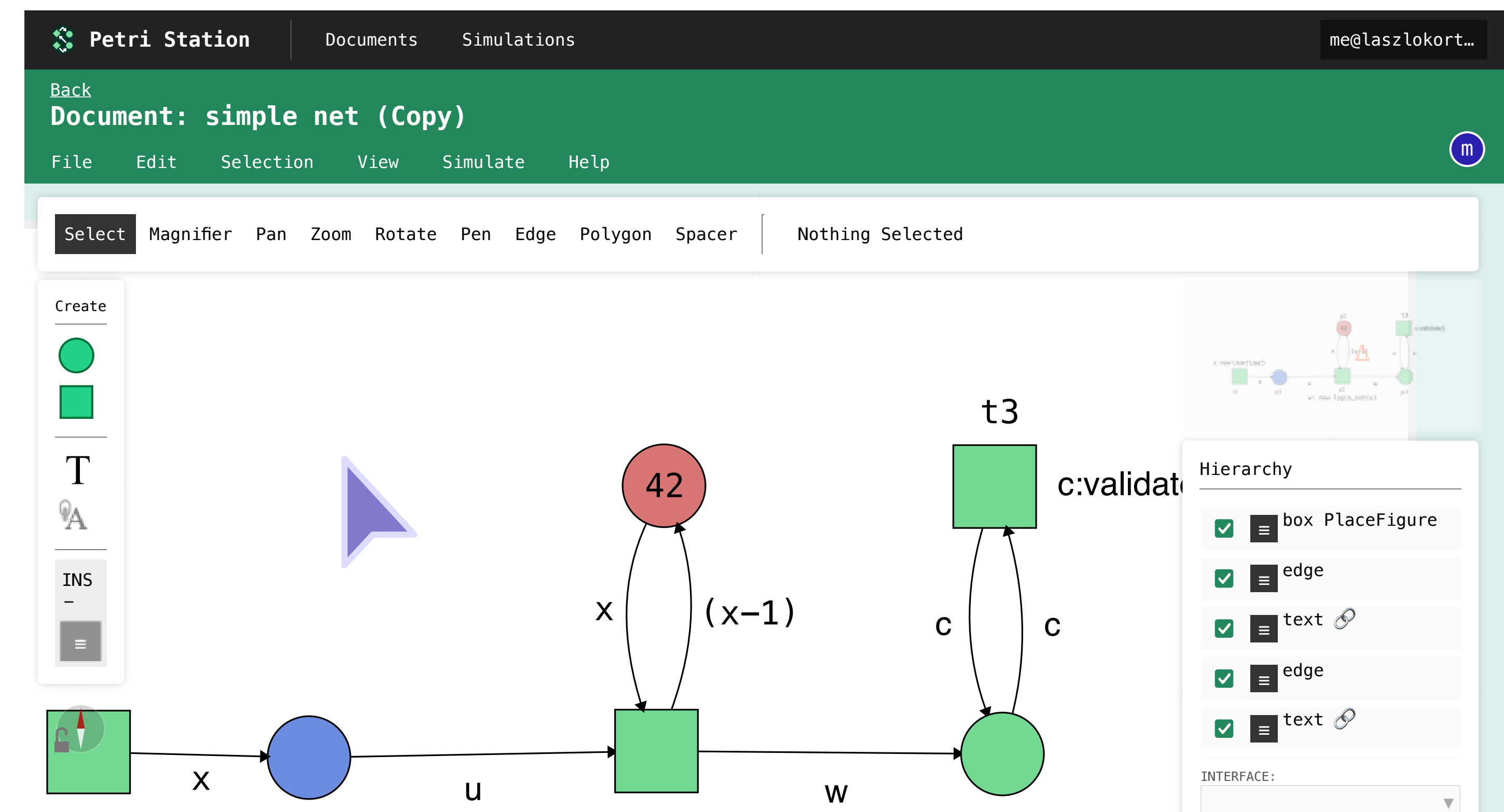
Figure 3: Screenshot of the editor user interface showing the toolbar (top), tool palette (left), mini-map (top right), element hierarchy (bottom right), and another user's collaborative cursor (center-left).
