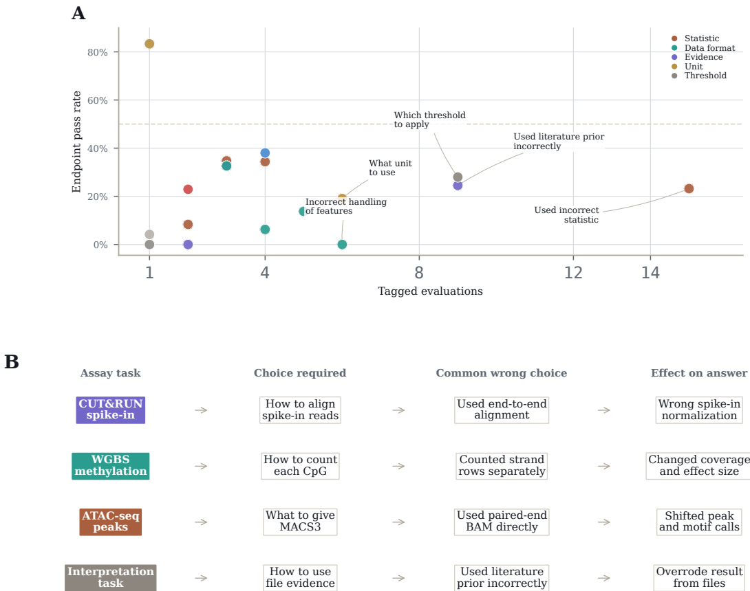
Figure 4: Many failures trace to plausible but wrong scientific choices. Panel A plots manually tagged failure behaviors by the number of reviewed evaluations carrying each behavior and the corresponding endpoint pass rate. Panel B shows representative assay choices where a plausible default changed the endpoint answer. Manual review covers 25/106 evaluations and is diagnostic rather than exhaustive.
