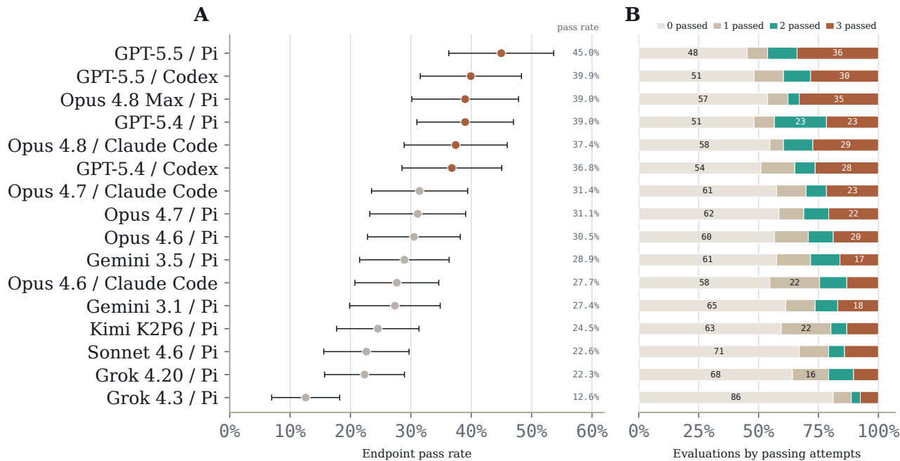
Figure 2: Endpoint pass rates across model-harness pairs. Panel A: endpoint pass rate across all 5,088 trajectories with 95% confidence intervals. Panel B: evaluation-level attempt outcomes over the same model order, partitioning the 106 evaluations for each model-harness pair by whether zero, one, two, or all three attempts passed.
