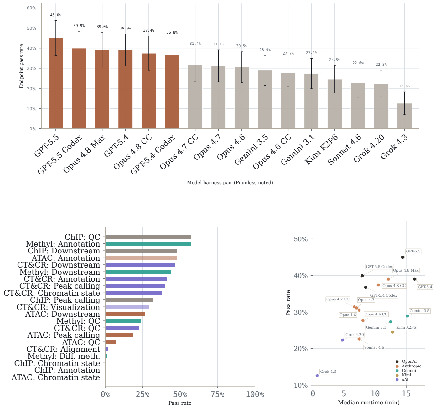
Figure 1: Topline benchmark performance. Top: evaluation-weighted pass rate by model-harness pair across all trajectories. The top panel shows Student t confidence intervals over evaluation-level mean pass rates. Bottom left: pass rate by assay and task family. Bottom right: pass rate against median runtime. Evaluation-level attempt statistics are reported in Table 2.
