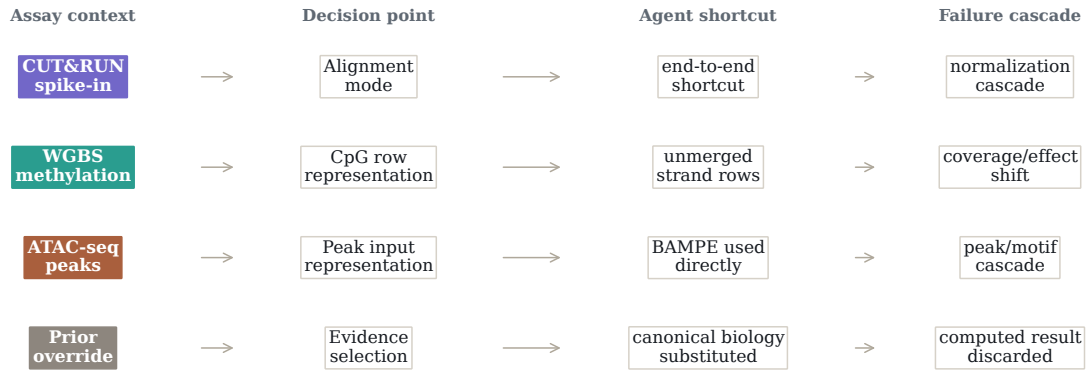
Figure 5: Reviewed failures concentrate in assay-specific decision traps. Panel A: frequency and severity of recurring error types from manual review; each point is an error type, with lower pass rates indicating harder traps. Panel B: representative assay decisions showing how a local shortcut can propagate into downstream endpoint failure. Manual review covers 25/106 evaluations and should be interpreted as diagnostic rather than exhaustive.
