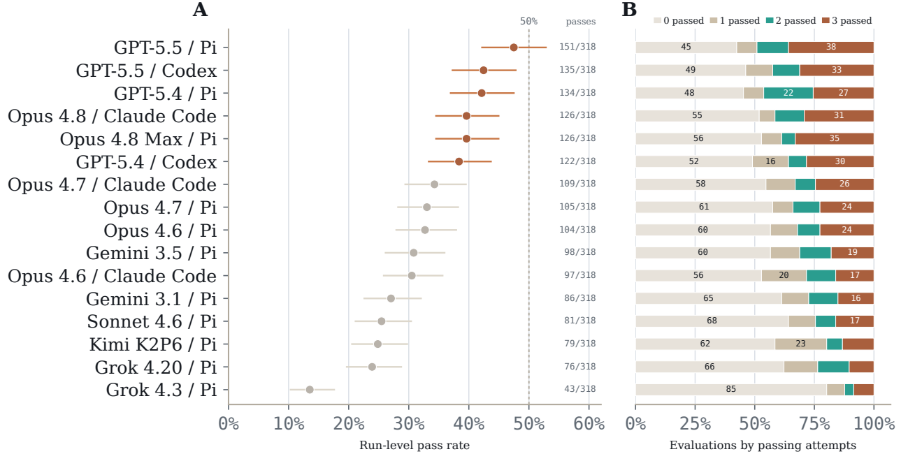
Figure 2: Endpoint accuracy and replicate outcomes across model-harness pairs. Panel A: run-level pass rate across all 5,088 parsed attempts, with Wilson confidence intervals and a 50% reference line. Panel B: evaluation-level replicate outcomes over the same model order, partitioning the 106 evaluations for each model-harness pair by whether zero, one, two, or all three attempts passed.
