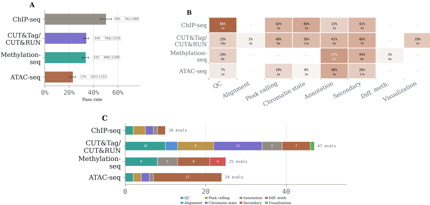
Figure 3: Performance varies by assay type. Panel A: run-level pass rate by assay type with Wilson confidence intervals and passing-attempt counts. Panel B: assay-by-task-category pass-rate heatmap; cell text reports pass rate and the number of evaluations in that cell. Panel C: evaluation-count composition by assay type, showing the task mix behind each assay summary.
