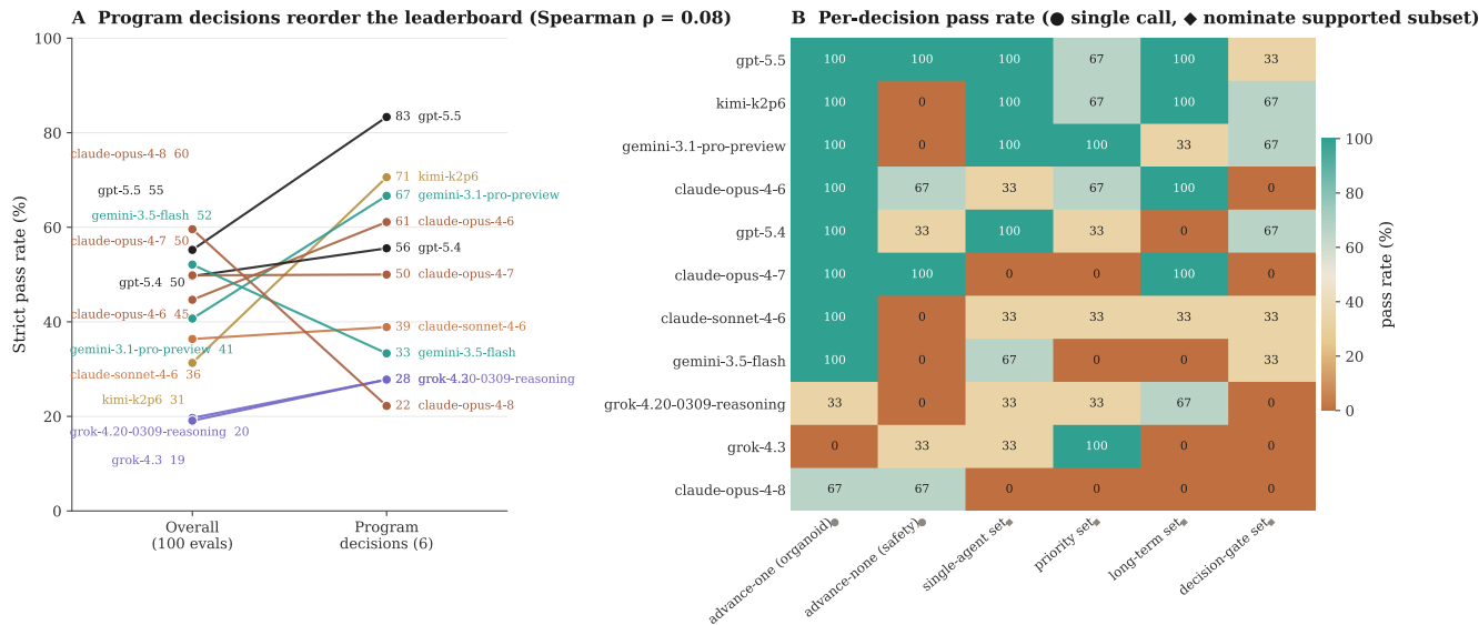
Figure 10: Aggregate accuracy does not predict program-decision competence. Pass rates on the six multi-evidence advancement decisions with complete Pi-harness model comparisons (up to 18 runs per model). (A) Endpoint pass rate on all 100 evaluations versus on the six program decisions; the integrative go/no-go calls reorder the leaderboard almost completely (Spearman \rho = 0.08 ), with the overall-best model, Claude Opus 4.8, falling to last and Kimi K2P6 rising from ninth to second. (B) Per-decision pass rate by model. The two single-compound calls (advance one, or hold; marked ●) are passed broadly, but the four tasks that require nominating the supported subset of models (marked with a diamond) separate the field; Claude Opus 4.8 fails all four.
