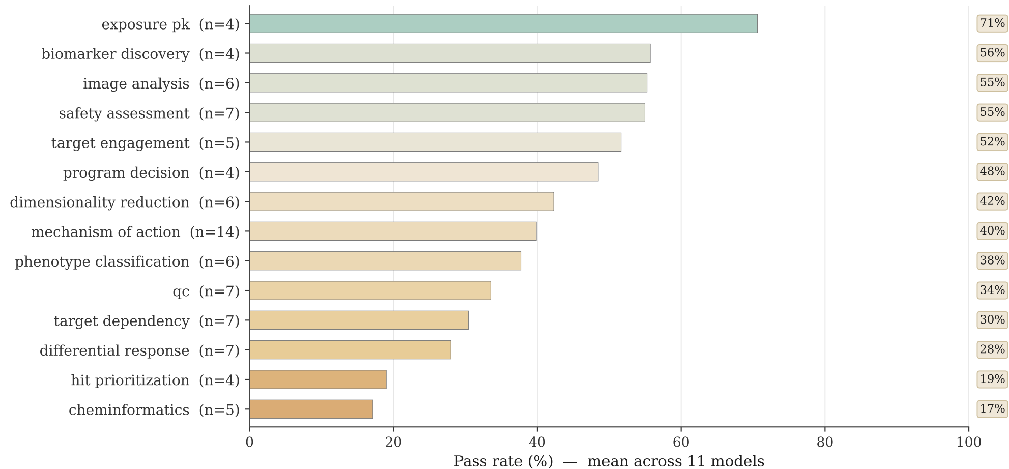
A Pass rate by task type (Pi harness; \geq 4 evals)
