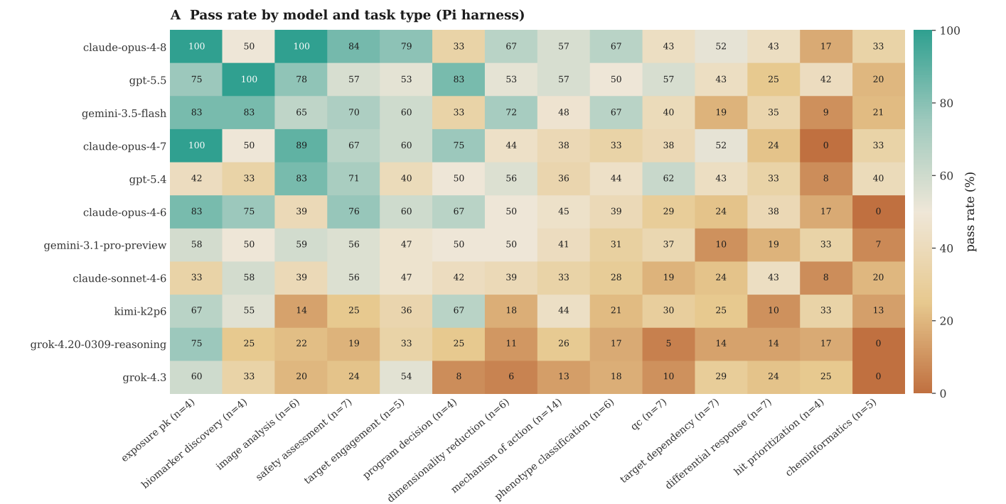
Figure 8: Pass rate by model and task type. Strict Pi-harness pass rate for each of the 11 models (rows, ordered by overall pass rate) across the task categories with at least four evaluations (columns, ordered easiest to hardest). Model quality sets the level across a row, but the hardest categories on the right stay low for every model.
