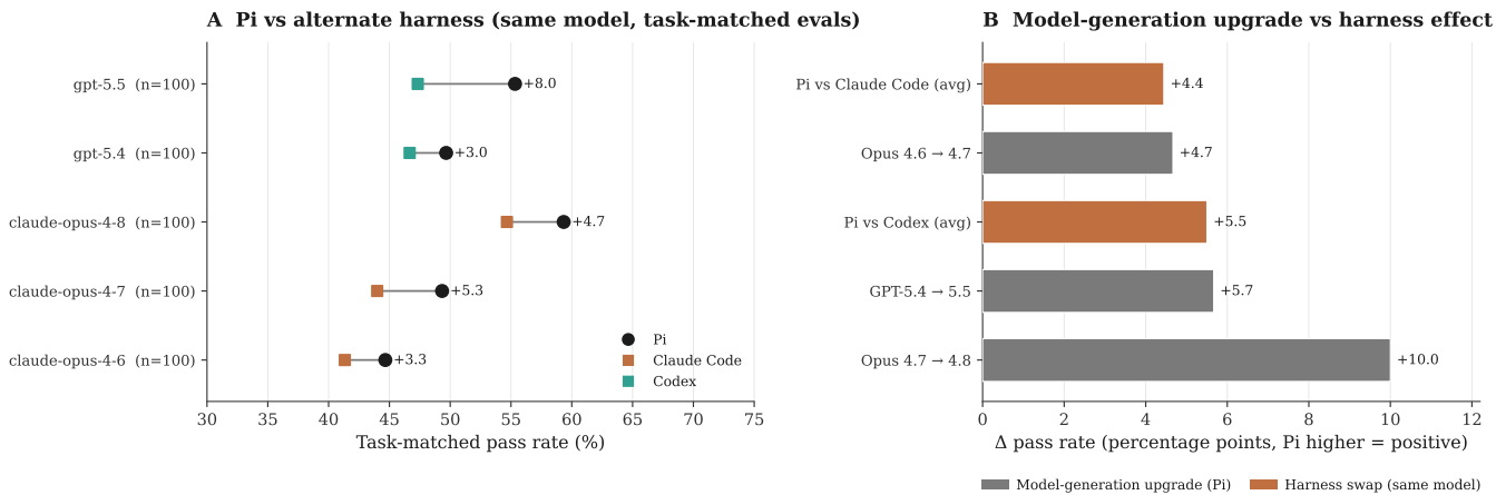
Figure 12: Harness choice is as consequential as a model-generation upgrade. (A) Task-matched pass rate on Pi versus the alternate harness for each model pair. Points are matched on the shared evaluation set; the labeled gap is the within-model Pi advantage in percentage points. (B) Head-to-head comparison of the Pi advantage over an alternate harness (terracotta) against the gain from a model-generation upgrade on Pi (grey). A harness substitution shifts pass rate by a margin comparable to upgrading one model generation, so reported scores should be interpreted as a property of the model-plus-harness, not the model alone.
