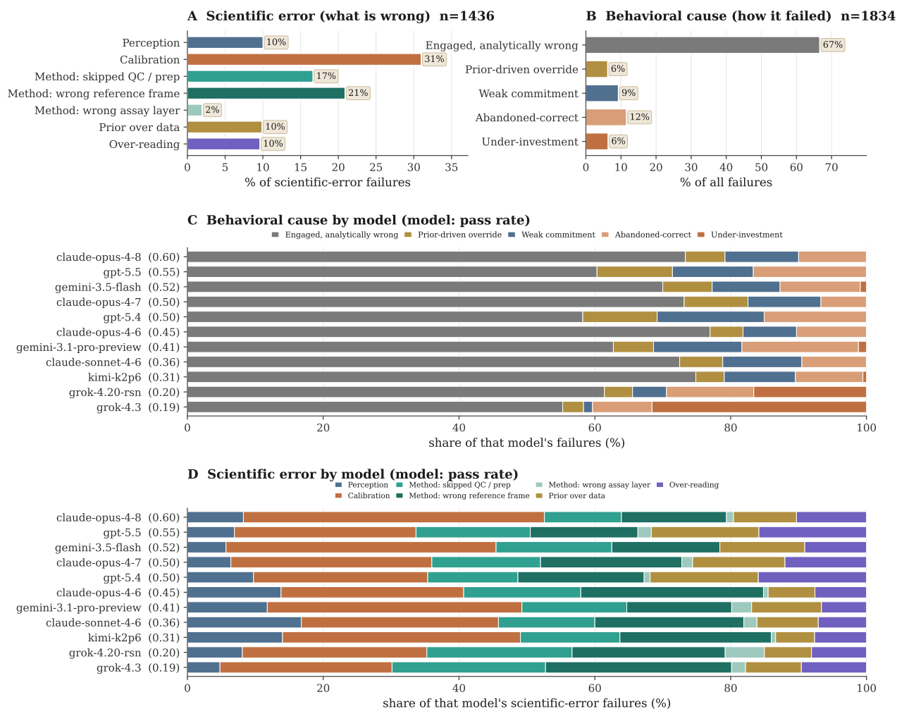
Figure 5: A two-axis failure taxonomy. All 1,834 failing (model, evaluation) runs on the Pi harness, labeled against each evaluation’s scientific intent and classified along two complementary axes. (A) The scientific-error axis (what is wrong with the answer) is dominated by method and calibration errors (71% combined), which are general analytical skills rather than domain knowledge; the method family resolves into a skipped-QC/preprocessing sub-mode and a larger wrong-reference-frame sub-mode. (B) The behavioral-cause axis (how the model failed) shows that a third of failures are non-analytical: a prior-driven override of the model’s own evidence, plus three process breakdowns (weak commitment, abandoned-correct, under-investment). (C) The behavioral mix is a model signature: under-investment dominates only the weakest model, while the strongest models fail almost entirely through engaged, analytically wrong reasoning. (D) The scientific-error mix, by contrast, is largely model-invariant: method and calibration errors dominate every model regardless of overall accuracy, so the kinds of scientific mistakes are shared across the frontier even as their rate falls (each bar normalized within that model’s scientific-error failures). A scientific-error × behavioral-cause cross-tabulation is provided in the supplement (fig_fm_crosstab).
