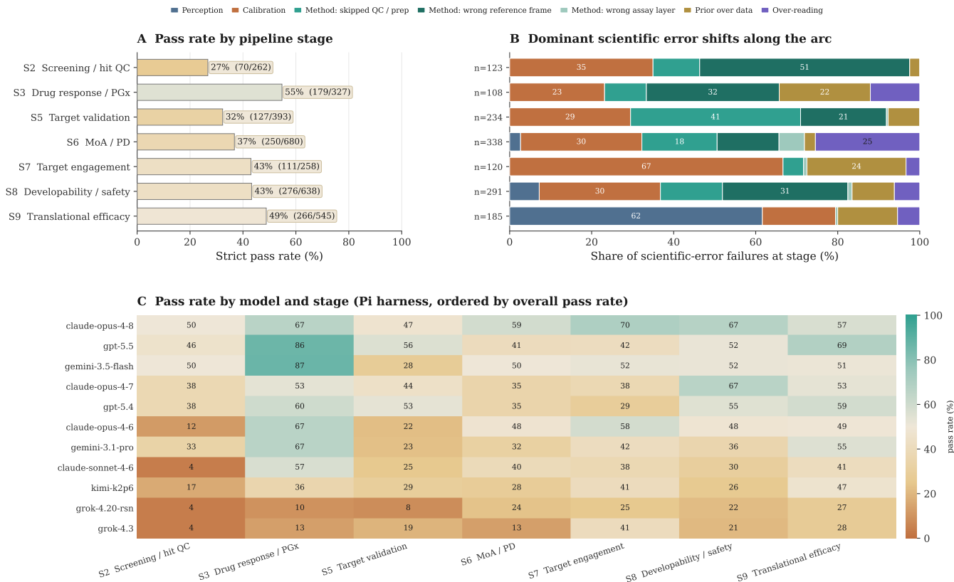
Figure 6: The dominant failure mode shifts across pipeline stages. Failing Pi-harness runs placed along the preclinical pharmacology arc. S1 disease-model and S4 target-genetics stages are omitted, since S1 is backed by too few evaluations and S4 is deferred to GenomicsBench. (A) Strict pass rate by stage. The two lowest are the early data-handling stages S2 (screening/QC) and S5 (causal target validation). (B) Scientific-error composition by stage, restricted to failures carrying a scientific error and using the same seven categories as Figure 5A. The dominant error shifts characteristically along the arc, from wrong reference frame at screening (S2) to skipped QC at target validation (S5), calibration at target engagement (S7), and perception at the image-heavy translational stage (S9), while calibration persists as a thread at every stage. (C) Strict pass rate for every model at each stage, ordered by overall pass rate. The overall ordering is largely preserved across stages, with two robust rearrangements: gemini-3.5-flash and gpt-5.5 lead at drug response (S3), and gemini-3.5-flash drops sharply at causal target validation (S5).
