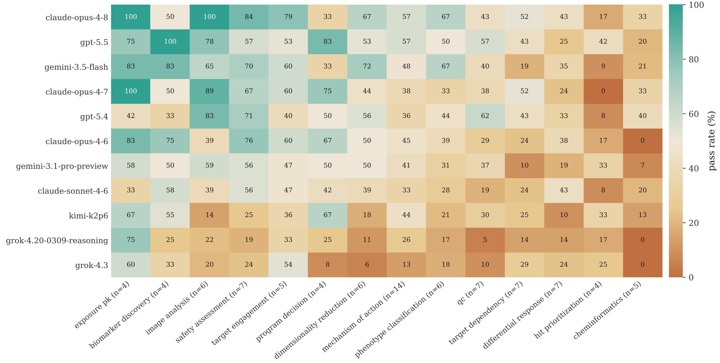
A Pass rate by model and task type (Pi harness)
