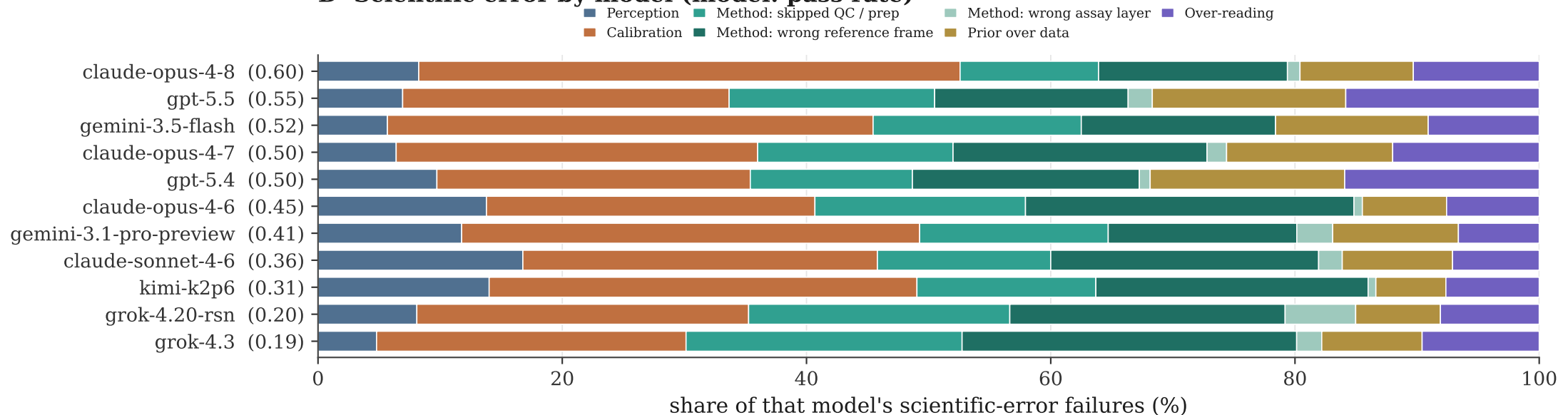
D Scientific error by model (model: pass rate)
