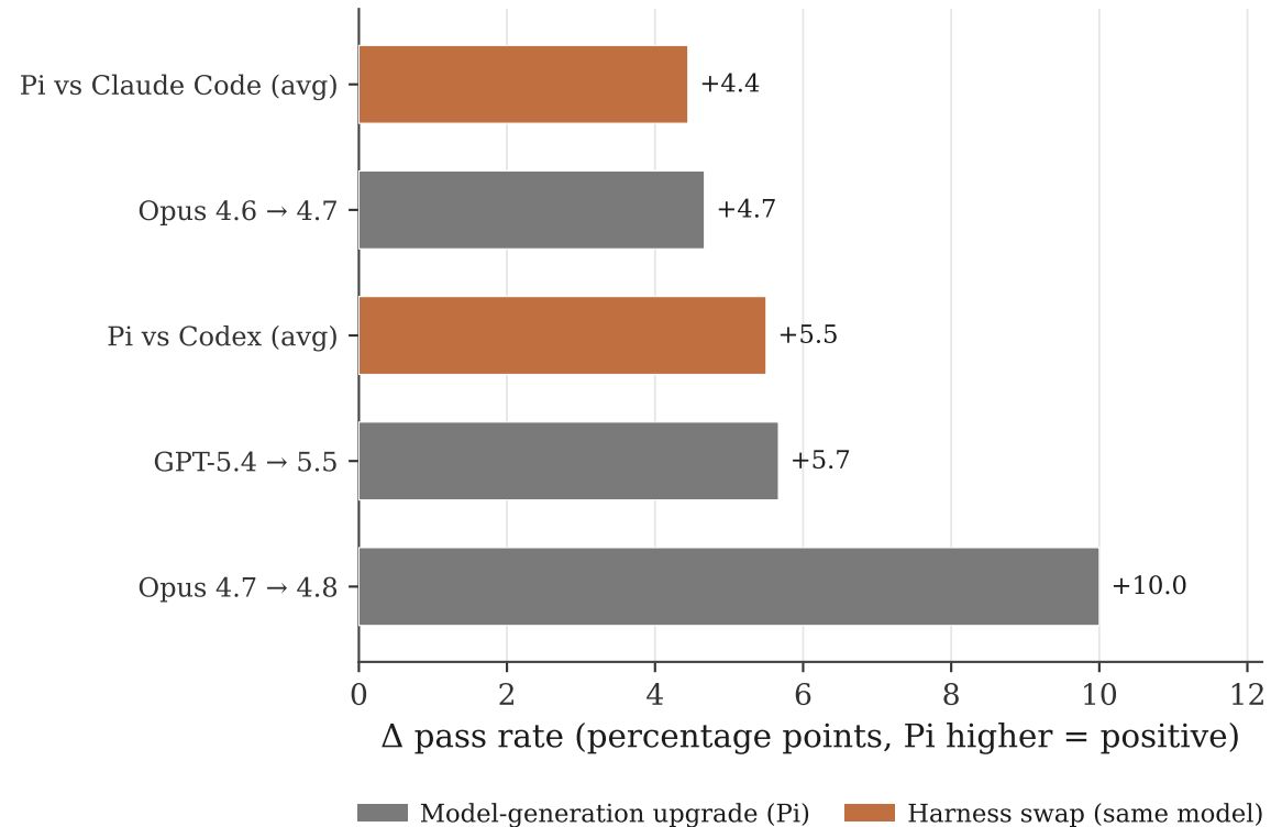
B Model-generation upgrade vs harness effect
