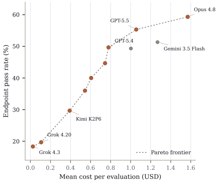
A Accuracy vs. cost
