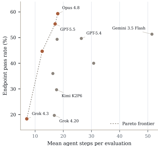
B Accuracy vs. steps
