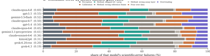
D Scientific error by model (model: pass rate)
