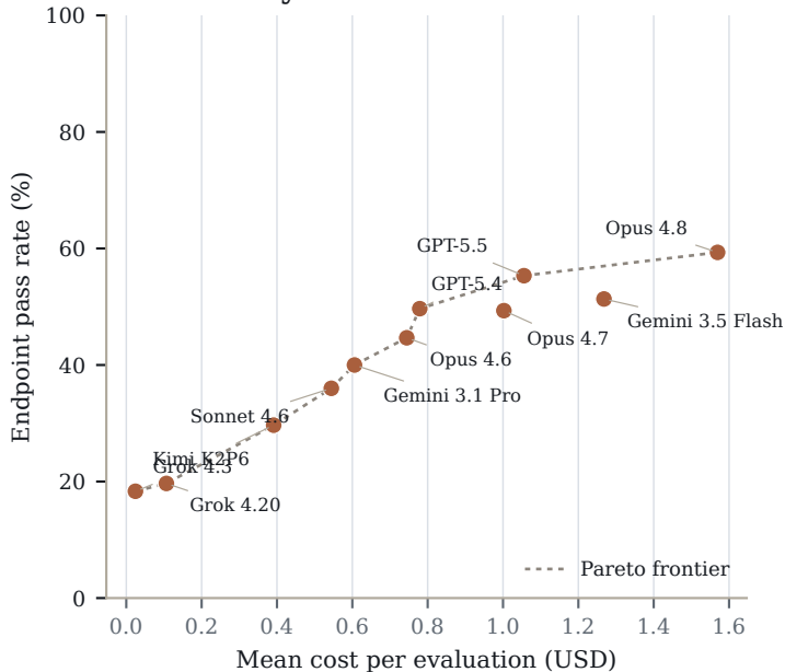
A Accuracy vs. cost
