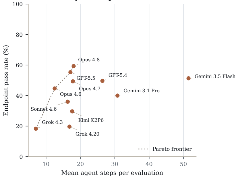
B Accuracy vs. steps
