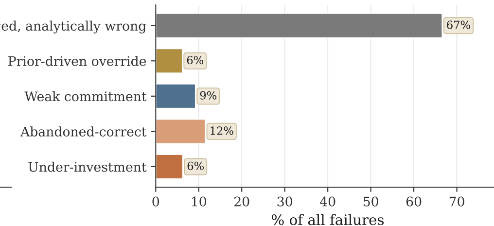
B Behavioral cause (how it failed) n=1834
