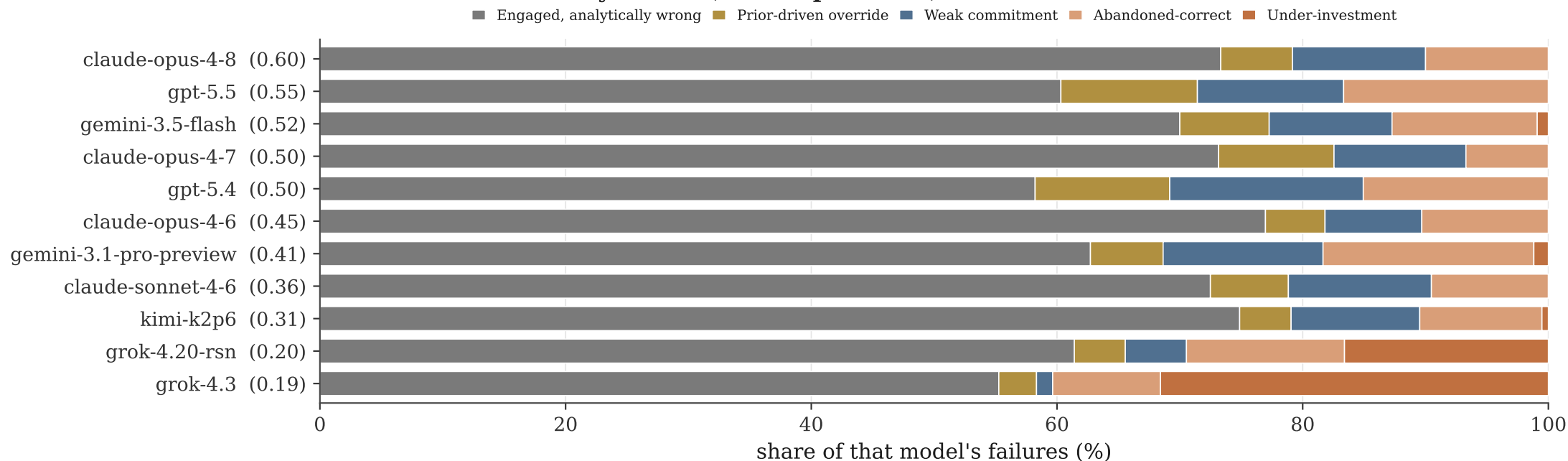
C Behavioral cause by model (model: pass rate)
