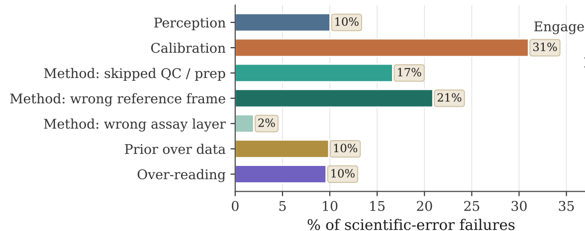
A Scientific error (what is wrong) n=1436
