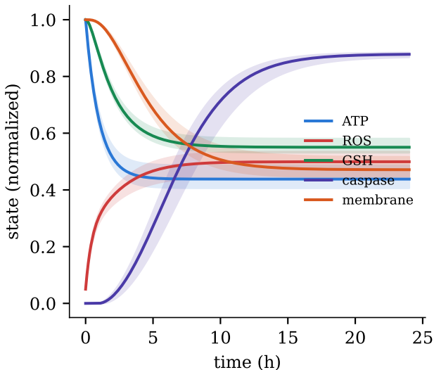
Digital twin at 37 \mu M rotenone (posterior band)
