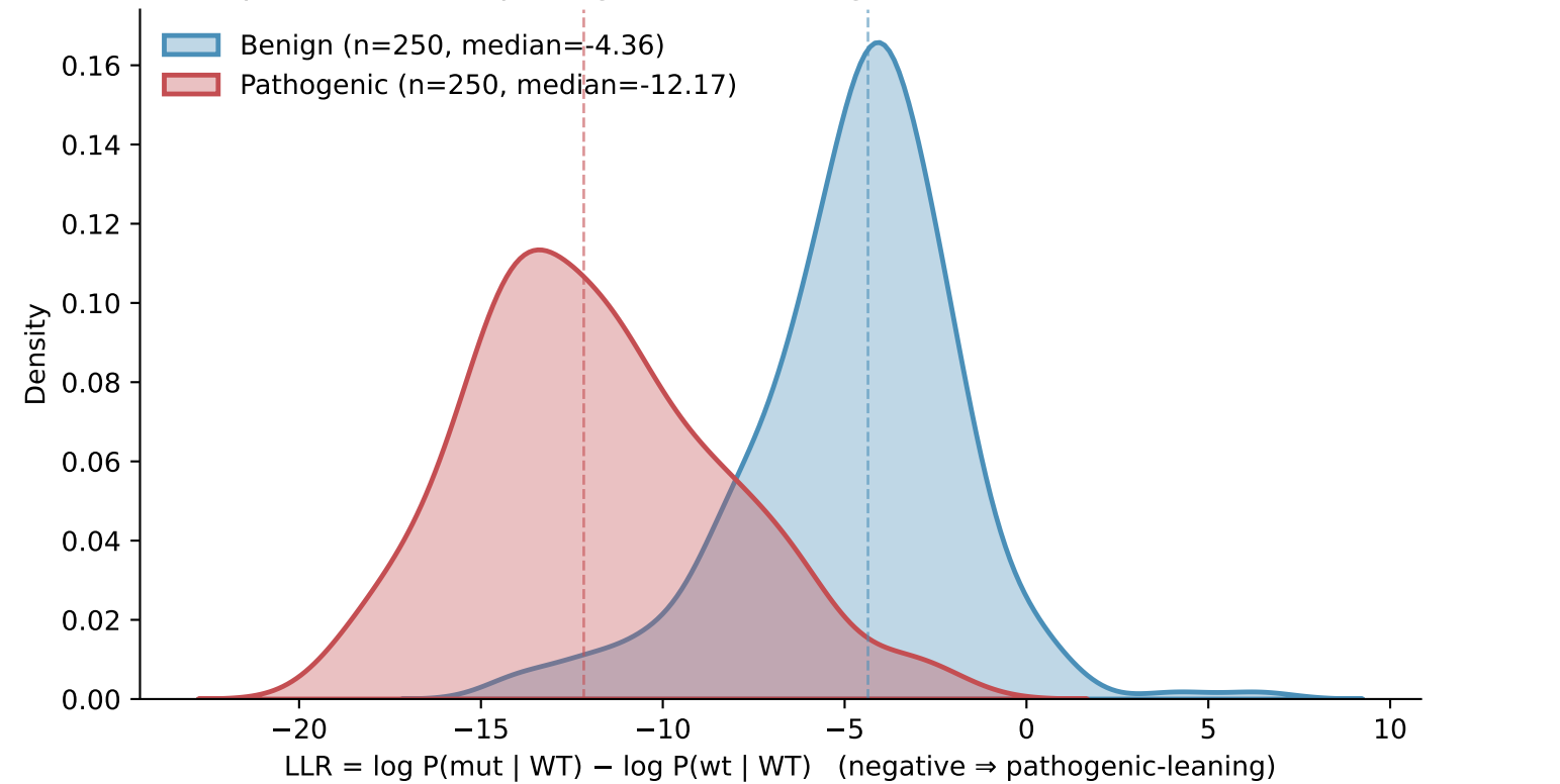
ESM-1b LLR separates ClinVar pathogenic from benign (AUROC = 0.930, 95% CI [0.906, 0.951])
