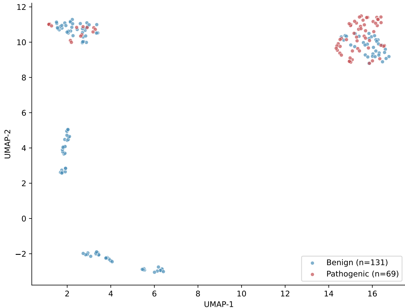
ESM-1b UMAP — BRCA1 ClinVar missense (n=200) — slide-1 fallback
