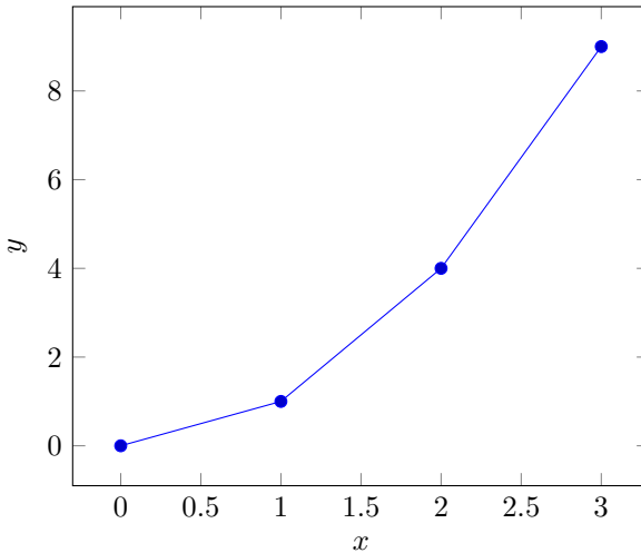
Figure 2.6: Explicit coordinates plotted with pgfplots.
