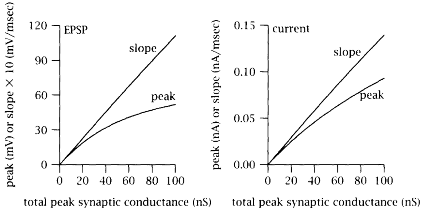
Figure 14.10 Plot of peak and slope of EPSP (left) and plot of peak and slope of EPSC (right) vs. synaptic conductance. Note that the slope is almost linearly related to the synaptic conductance whereas the peak voltage and current associated with the EPSP show pronounced nonlinear summation. (From simulations by Erik Cook.)
