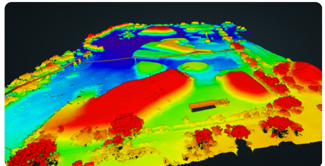
Volumetric Analysis for Coal and Sand Stockpiles
