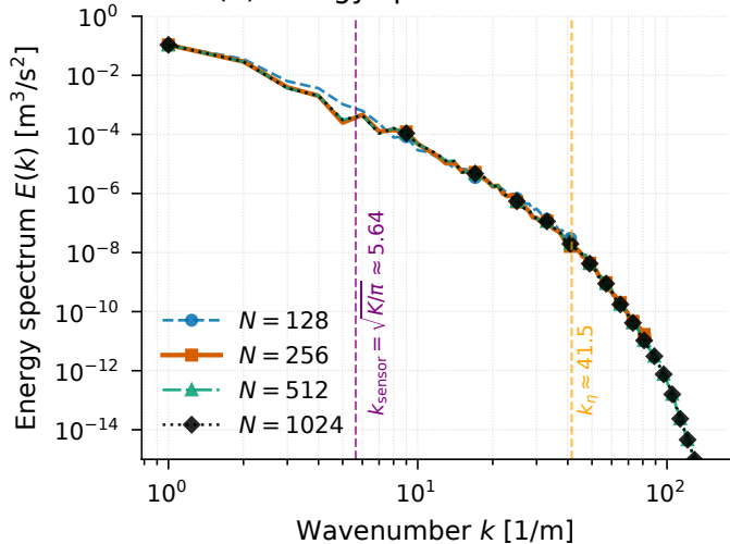
(b) Energy spectrum at t = 5 s
