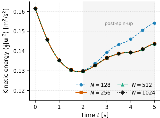
(a) Kinetic energy time series
