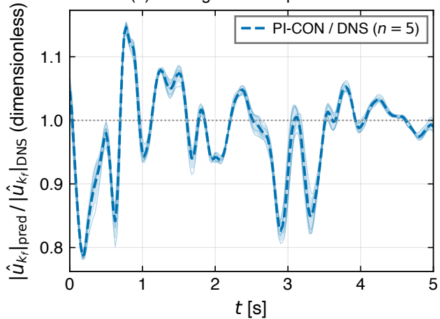
(a) Forcing-mode amplitude ratio
