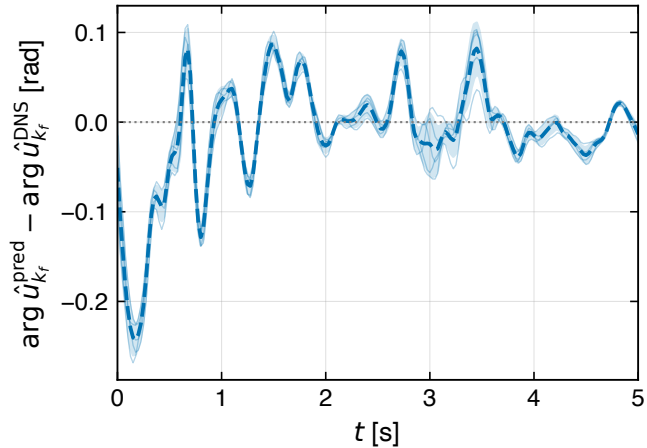
(b) Forcing-mode phase error
