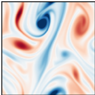
DNS
