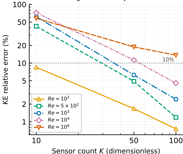
Sensor budget versus Reynolds number
