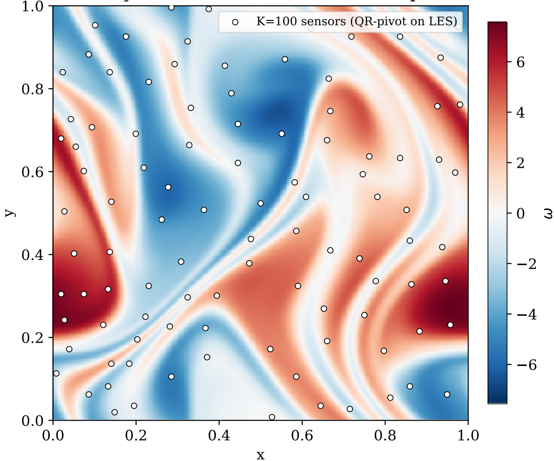
LES vorticity \omega at t = 50 with K=100 sensor placement
