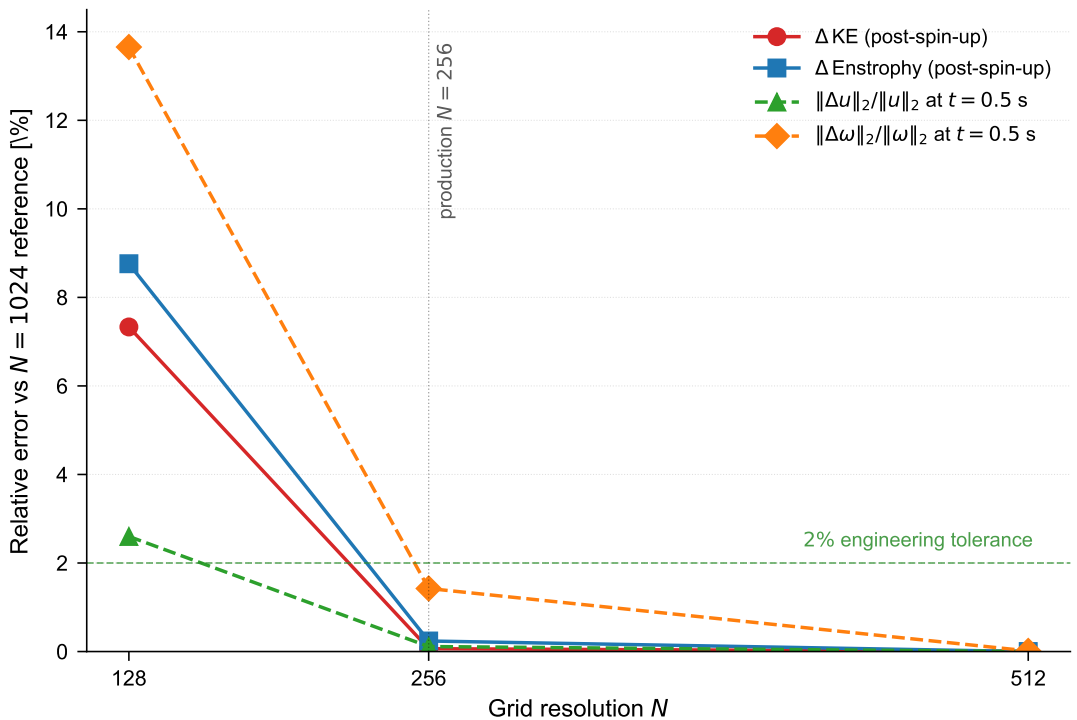
Grid convergence ( Re = 10^4 , T = 5 s)
