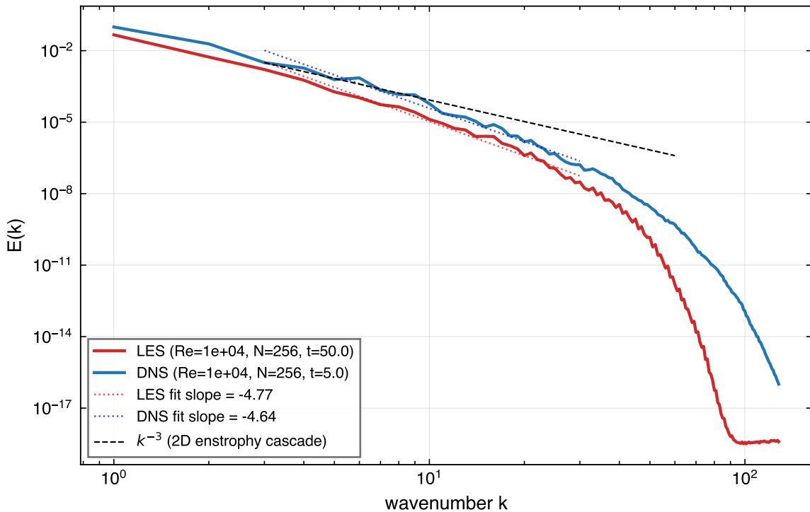
Late-time energy spectrum (radial)
