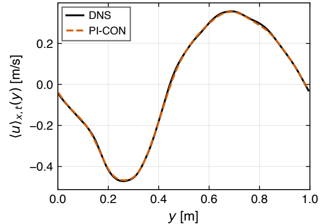
(a) Mean streamwise profile
