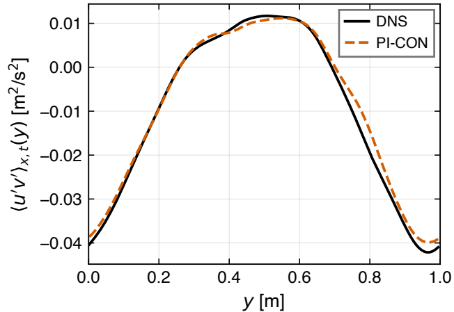
(b) Reynolds shear stress
