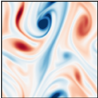
DNS
