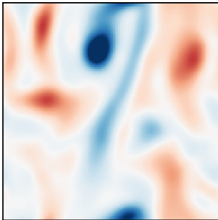
K = 100
