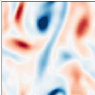
K = 400
