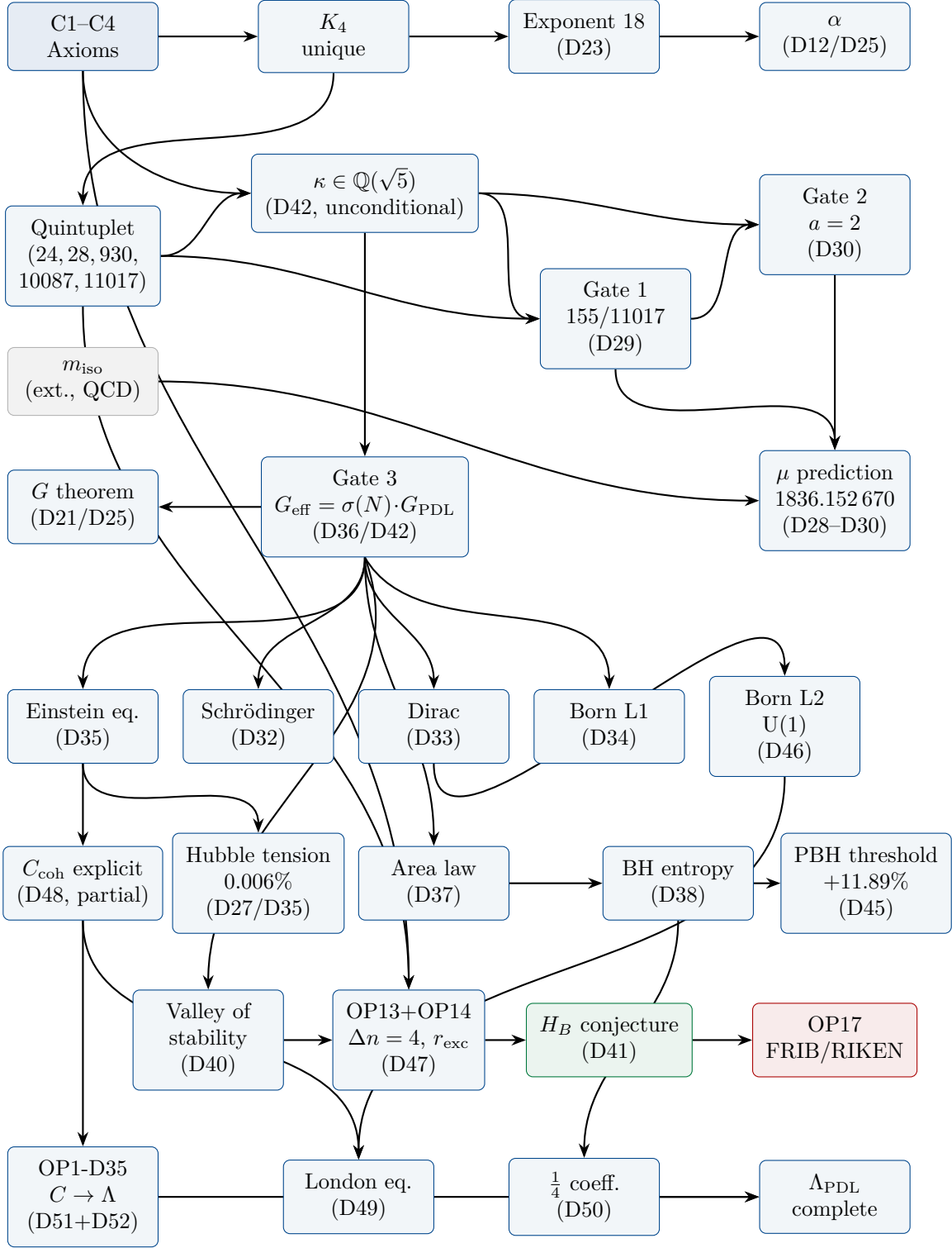
Figure 1: Critical-path dependency map of the PDL programme (v20). Blue nodes: unconditional theorems. Green: conjectures. Red: open problems. Grey: unique external input ( m_{\text{iso}} ). The quantum dynamics layer (Schrödinger, Dirac, Born L1, Born L2/U(1), London equation), the nuclear stability layer (OP13, OP14, valley of stability), the black hole thermodynamics layer (area law, Bekenstein–Hawking, \frac{1}{4} coefficient), and the cosmological leakage layer ( C \rightarrow \Lambda_{\text{PDL}} ) are all complete. The causal chain C1\text{--}C4 \rightarrow \Lambda_{\text{PDL}} is fully closed; D53 provides the independent numerical synthesis.
