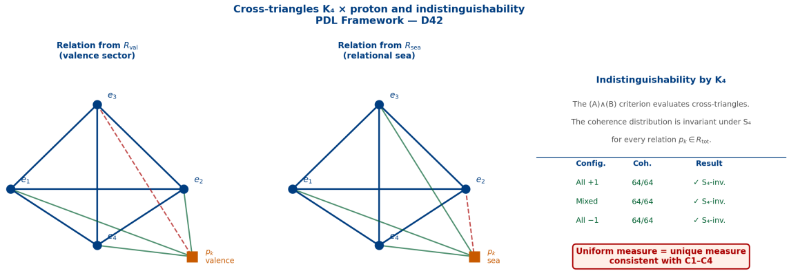
Figure 2: Cross-triangles between an external K_4 and proton relations. Left: a valence relation p_k \in \mathcal{G}_{\text{val}} . Centre: a sea relation p_k \in \mathcal{G}_{\text{sea}} . Right: exhaustive verification table showing that all 64 signed K_4 configurations are S_4 -invariant. The external K_4 cannot distinguish valence from sea relations via cross-triangles.
