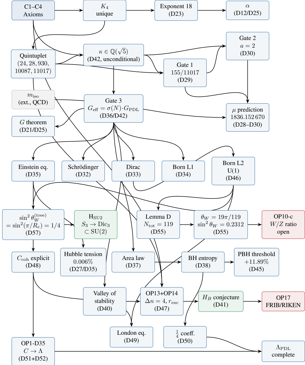
Figure 1: Critical-path dependency map of the PDL programme (v23). Blue nodes: unconditional theorems. Green: conjectures. Red: open problems. Grey: unique external input ( m_{\text{iso}} ). The quantum dynamics layer (Schrödinger, Dirac, Born L1, Born L2/U(1), London equation), the nuclear stability layer (OP13, OP14, valley of stability), the black hole thermodynamics layer (area law, Bekenstein–Hawking, \frac{1}{4} coefficient), the cosmological leakage layer ( C \rightarrow \Lambda_{\text{PDL}} ), and the electroweak sector ( \theta_W = 19\pi/119 , D55) are all complete theorems of C1–C4. The causal chain C1–C4 \rightarrow \Lambda_{\text{PDL}} is fully closed; the electroweak gauge geometry is structurally derived. Remaining open: W/Z mass ratio (OP10-c) and experimental lattice QCD test of \Delta m_{\text{iso}} (OP10-d).
