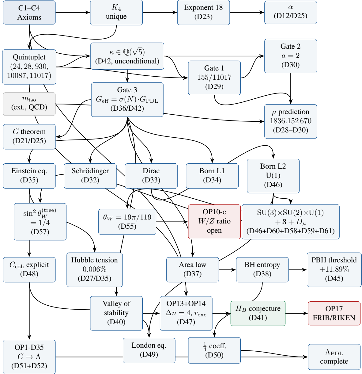
Figure 1: Critical-path dependency map of the PDL programme — foundational chain (v31). Blue: unconditional theorems. Green: conjectures. Red: open problems. Grey: unique external input ( m_{\text{iso}} ). The quantum dynamics layer (Schrödinger, Dirac, Born, London), nuclear stability, black hole thermodynamics, and cosmological constant are complete theorems of C1–C4. The gauge sector node (bottom right) is a summary; the full derivation chain K_4 \rightarrow D_\mu is detailed in Figure 2.
