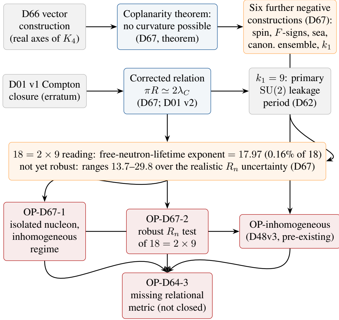
Figure 5: D67 dependency chain: coplanarity, the corrected wave-closure relation, and the isolated-nucleon open problems (new in v31). Blue: unconditional theorems. Orange: documented negative results, including one reported as a motivated but not yet robust numerical lead rather than an established result. Red: open problems. Grey: inputs from D66 and D01, and the pre-existing Open Problem OP-inhomogeneous (D48v3). D67 proves the coplanarity theorem, closing the D66 vector-construction route, and reports six further negative constructions; independently, correcting a transcription erratum in D01 (the proton Compton-closure relation) leads, via the SU(2)-period identity k_1 = 9 already established in D62, to a striking connection between the topological exponent 18 and the free-neutron lifetime, not yet robust under realistic uncertainty. Both threads converge on the isolated-nucleon open problems OP-D67-1 and OP-D67-2, and ultimately on the still-open OP-D64-3.
