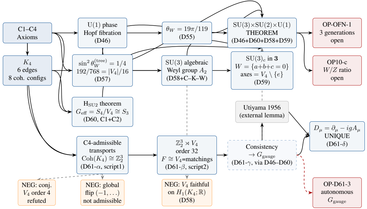
Figure 2: Gauge sector dependency map of the PDL programme (v28). Blue solid: unconditional theorems. Blue dashed: consistency result (arrow \gamma of D61: the transport structure is consistent with G_{\text{gauge}} , but this arrow relies on D46–D60 rather than being a new derivation). Grey: external lemma (Utiyama 1956). Red: open problems. Orange: documented negative results (scientifically informative). The four arrows of the D61 causal chain are labelled \alpha – \delta . \alpha : C4 forces \text{Coh}(K_4) \cong \mathbb{Z}_2^3 (2048 checks). \beta : V_4 acts faithfully on \mathbb{Z}_2^3 by automorphisms, F \cong V_4 fixed by the three perfect matchings (288 checks). \gamma : consistency with G_{\text{gauge}} (theorem via D46–D60). \delta : D_\mu = \partial_\mu - igA_\mu unique, by Utiyama. The complete gauge sector — group, representations, and dynamics — is derived from C1–C4 with no variational postulate and no free parameter at the structural level.
