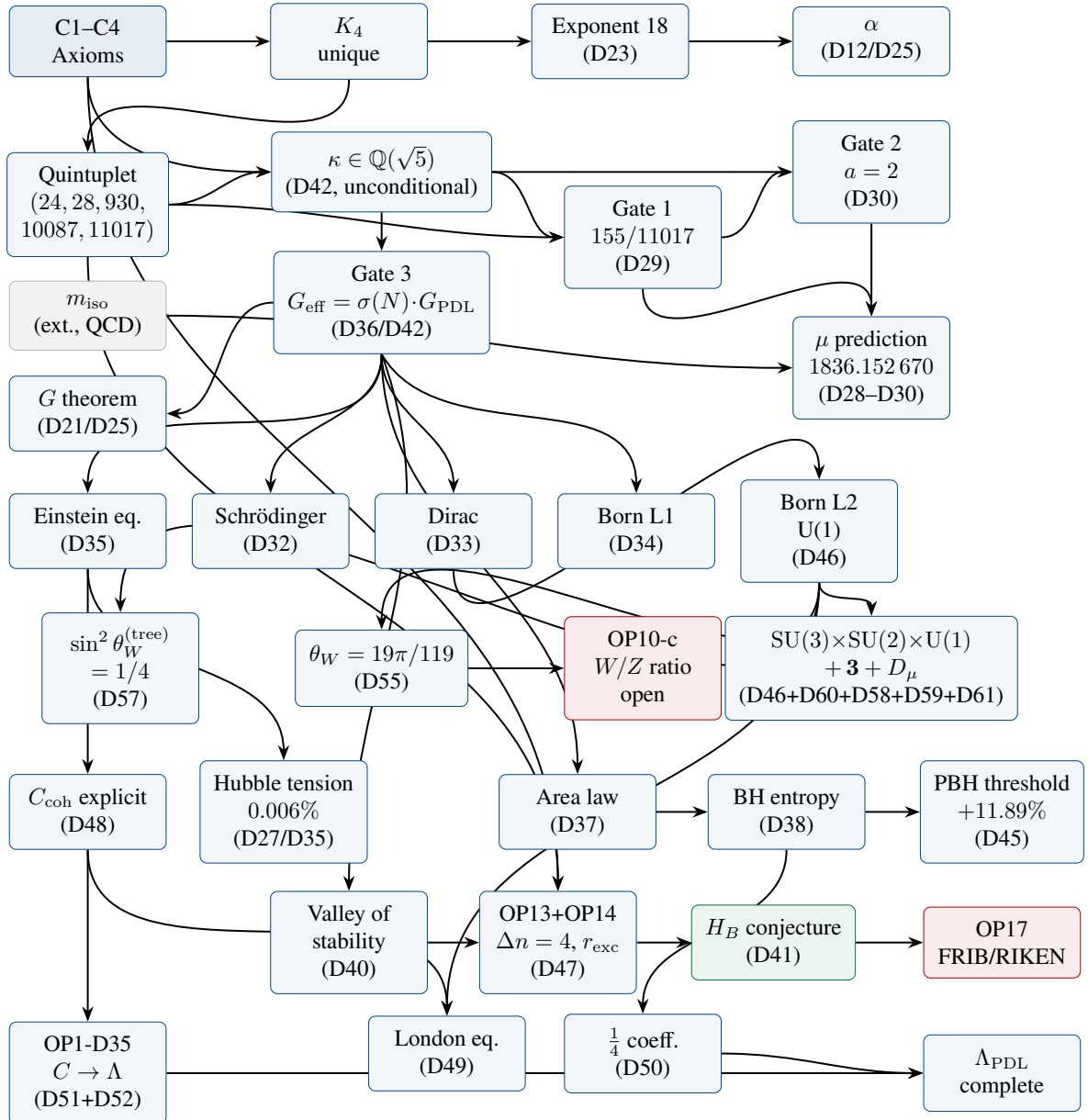
Figure 1: Critical-path dependency map of the PDL programme — foundational chain (v28). Blue: unconditional theorems. Green: conjectures. Red: open problems. Grey: unique external input ( m_{\text{iso}} ). The quantum dynamics layer (Schrödinger, Dirac, Born, London), nuclear stability, black hole thermodynamics, and cosmological constant are complete theorems of C1–C4. The gauge sector node (bottom right) is a summary; the full derivation chain K_4 \rightarrow D_\mu is detailed in Figure 2.
