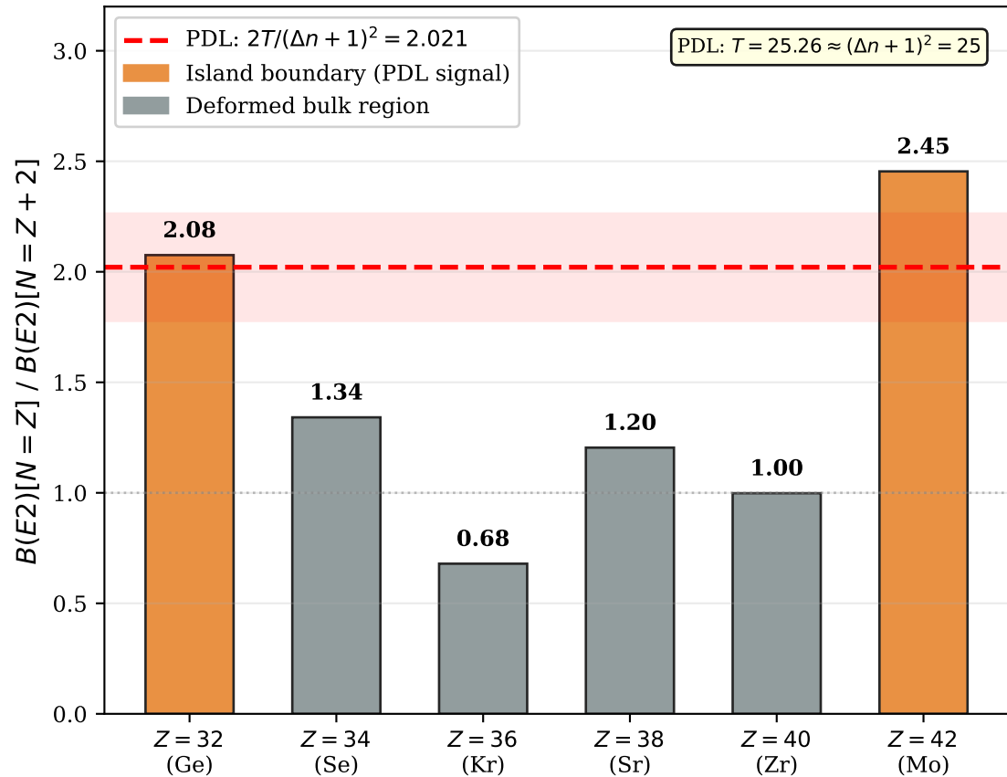
(b) Ratio B(E2)[N = Z]/B(E2)[N = Z + 2] vs PDL prediction
