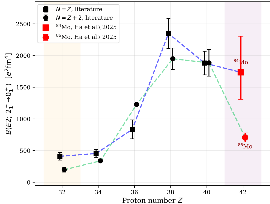
(a) B(E2; 2_1^+ \rightarrow 0_1^+) systematics along N = Z and N = Z + 2
