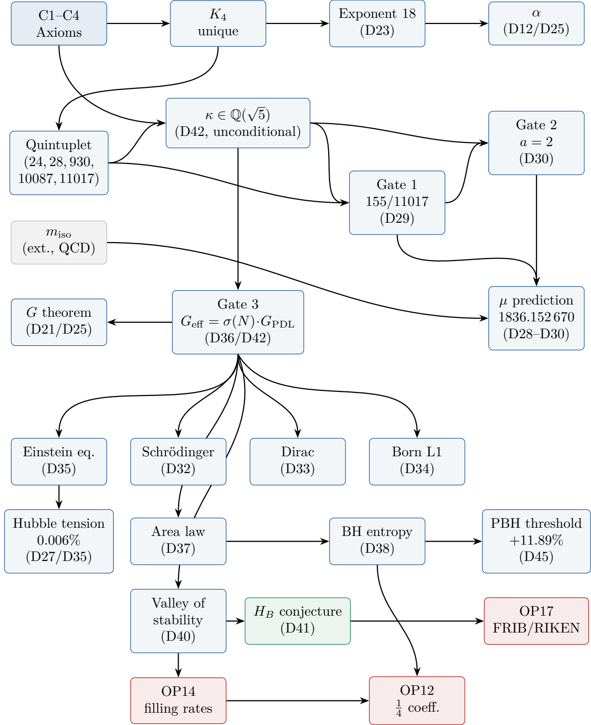
Figure 1: Critical-path dependency map of the PDL programme (v17). Blue nodes: unconditional theorems. Green: conjectures. Red: open problems. Grey: unique external input ( m_{\text{iso}} ). All previously conditional results are now solid arrows. D45 (PBH threshold) is the first falsifiable astrophysical confrontation.
