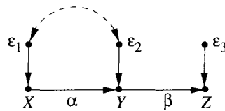
Figure 5.2 A testable model containing unidentified parameter ( \alpha ).
