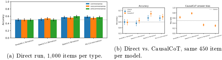
Fig. 3: Accuracy with 95% confidence intervals. The dashed line marks chance (0.5). No model is clearly less accurate on anti-commonsensical items, and reasoning first clearly improves accuracy only for Qwen2.5-7B-Instruct.
