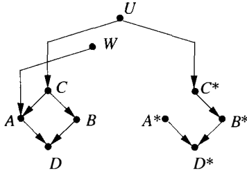
Figure 7.2 Twin network representation of the firing squad.
