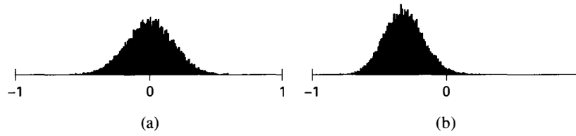
Figure 8.5 (a) The prior distribution of \text{ACE}(X \rightarrow Y) induced by flat priors over the parameters v_{CR} . (b) The distribution for \text{ACE}(X \rightarrow Y) induced by skewed priors over the parameters.
