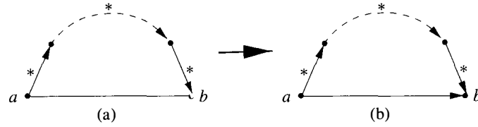
Figure 2.2 Illustration of R_2 in step 3 of the IC* algorithm.
