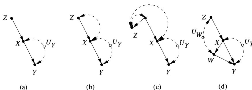
Figure 7.8 Z is a proper instrumental variable in the (linear) models of (a), (b), and (c), since it satisfies Z \perp\!\!\!\perp U_Y . It is not an instrument in (d) because it is correlated with U_W , which influences Y .
