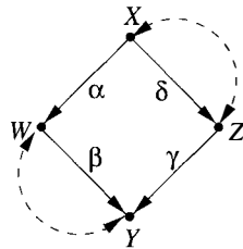
Figure 5.10 Graphical identification of \alpha , \beta , and \gamma .
