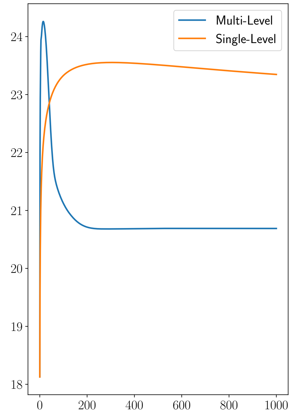
PSNR function w.r.t iterations
