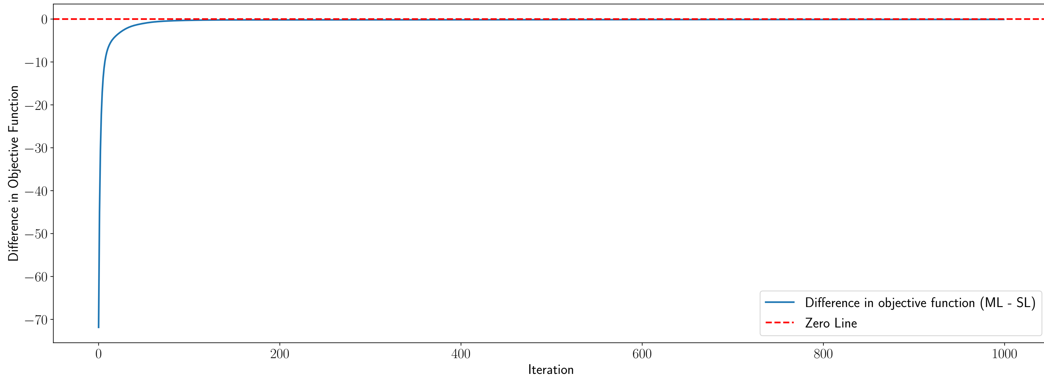
Difference in Objective Function between ML and SL Last value: -0.0830
