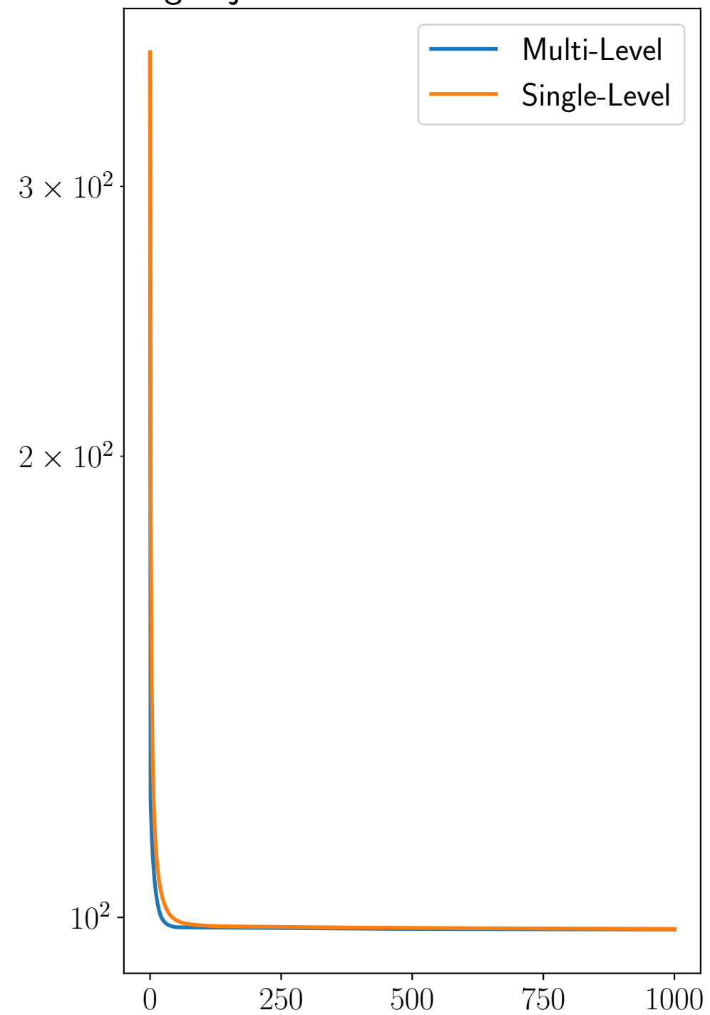
Log objective function w.r.t iterations
