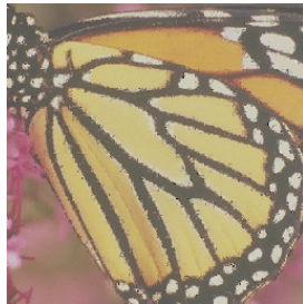
Observation Reconstructed (FR) Reconstructed (BCD) Reconstructed (BCD cond) PSNR: 10.76 PSNR: 22.56 PSNR: 15.09 PSNR: 15.49
