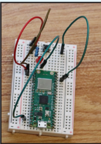
Attacker Raspberry Pi Pico W: One button (on/off) and red status LED
