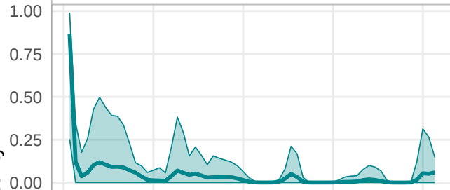
Cluster 2
