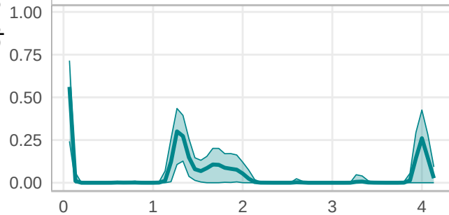
Cluster 5
