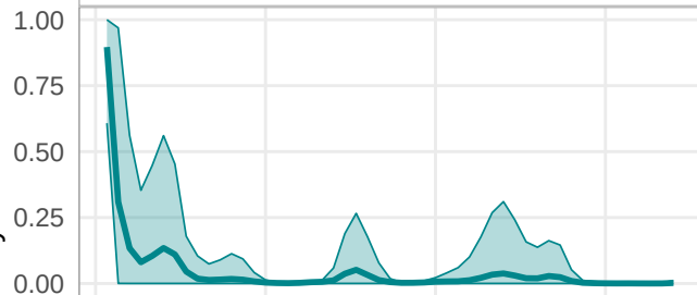
Cluster 2
