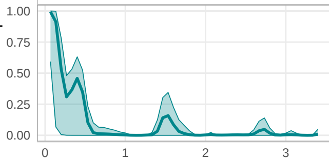
Cluster 5
