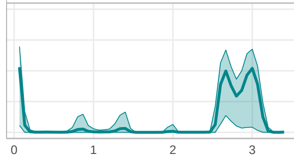
Cluster 4
