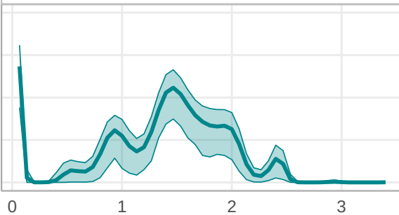
Cluster 3
