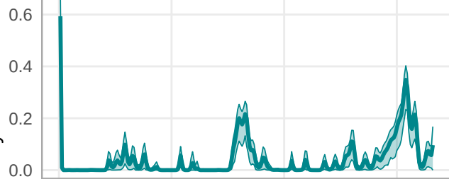
Cluster 5
