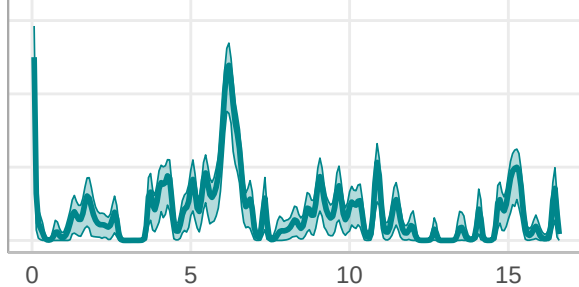
Cluster 3
