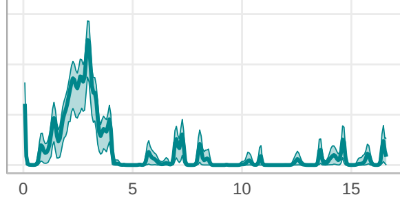
Cluster 4
