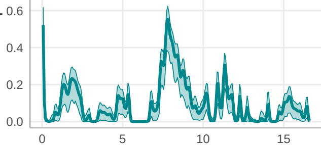
Cluster 5
